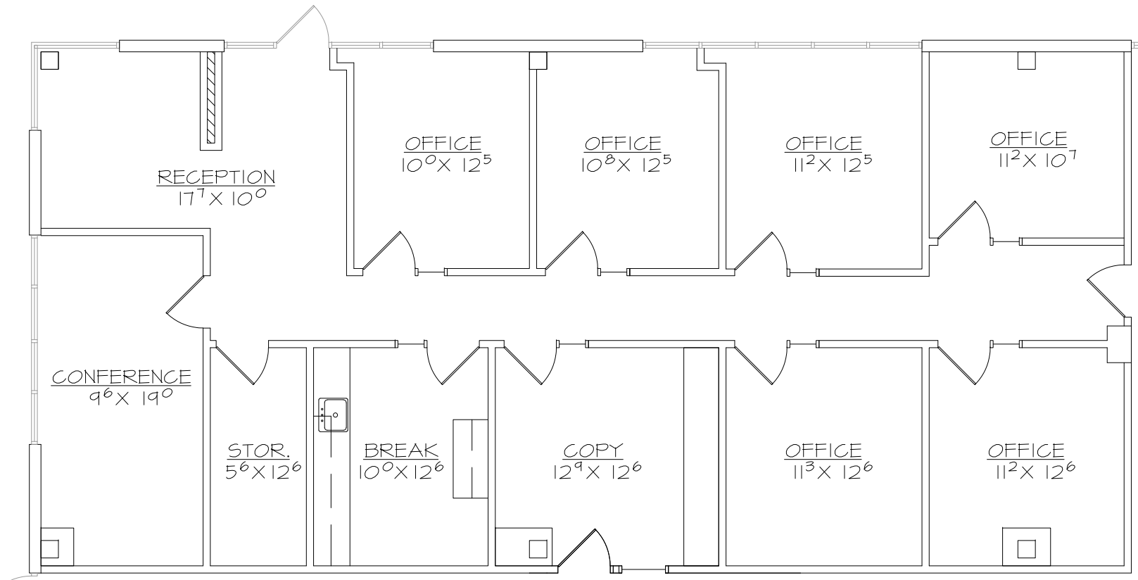
First Floor Overall Plan
